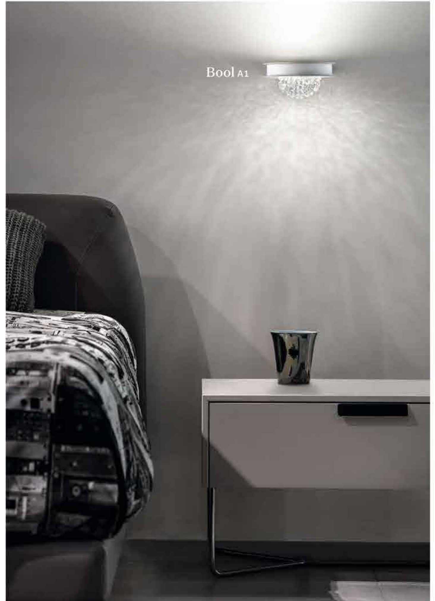
Bool
